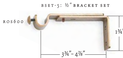
BSET-5: 1/2" BRACKET SET
