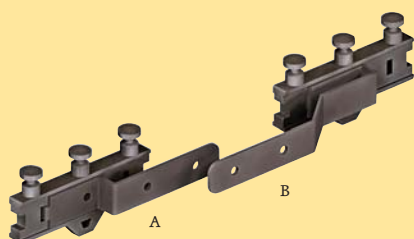
A) MASTER CARRIER WITH STANDARD ARM
