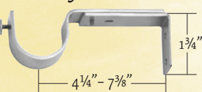
BSET-1: 1" BRACKET SET
